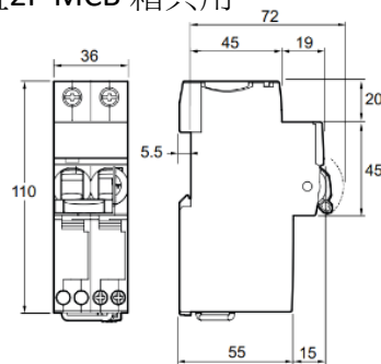
iC60H2 RCBO
