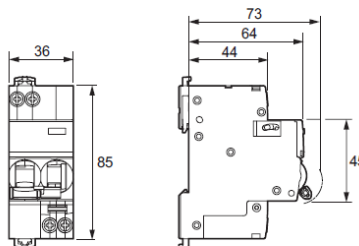
Residual current devices 1P+N
